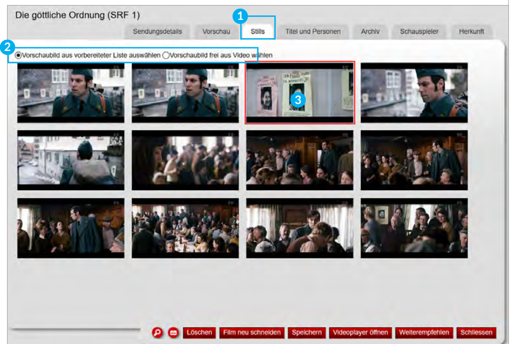
Abb. 7.15 Register Stills
